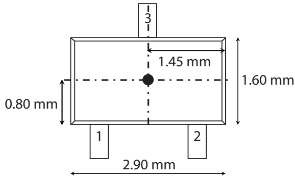
8.1 SOT-23-3 Package
